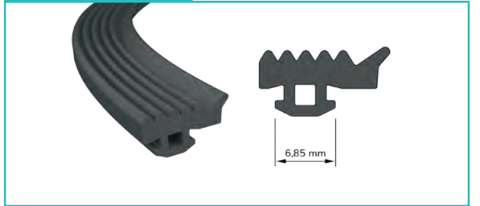
Dayama Fitili Seal Rest
