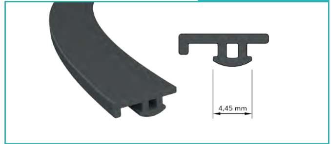
Çakma Conta Nailing Joint
