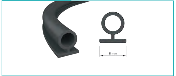
Omega Fitol 6 mm. Omega Seal 6 mm.
