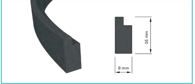
Genel Fitol General Seal
