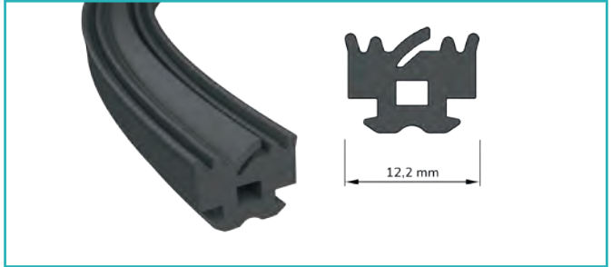
Dayama Fiteli Seal Rest
