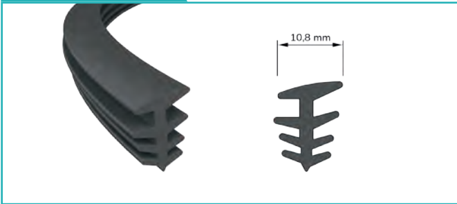
Tirnaklı Cam Fiteli Spiked Glass Seal
