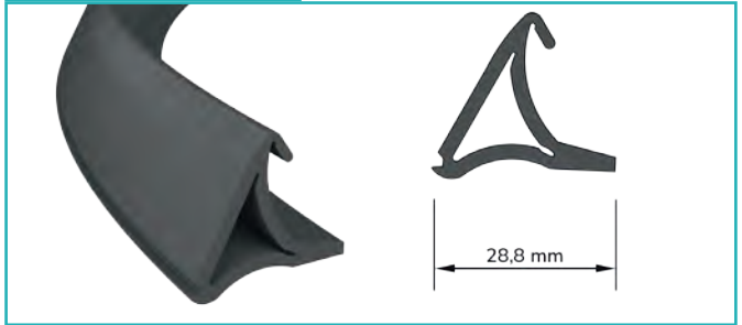
Orta Kanat Fitili Middle Wing Seal
