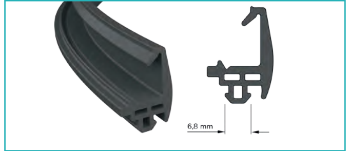
Tozluk Fıtlı Powder Seal
