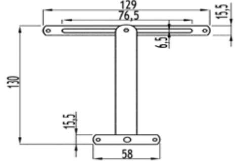
VASISTAS MAKAS VASISTAS OPENING MECHANISM
