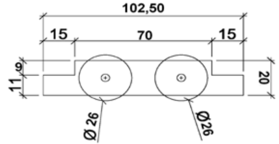
TEK TEKER PİRİNÇ RULMAN
