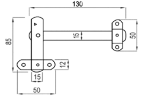
3 KADEMELİ MAKAS VASISTAS OPENING MECHANISM
